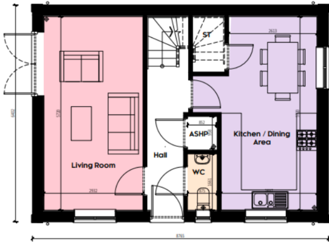
Ground Floor Plan 1 : 100
